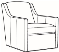
Kendrick / L545-05 Leather Chair (29W) Outside: 29W x 36.5D x 34H Inside: 22.5W x 21D
